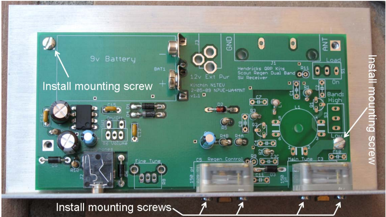
Figure 32. Temporarily mount PC Board to the chassis and C3, C5 to the front panel
